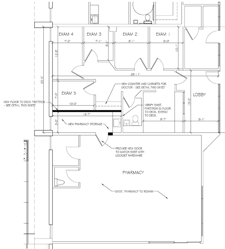
NEW WORK FLOOR PLAN SCALE: 1/4" = 1'-0"
